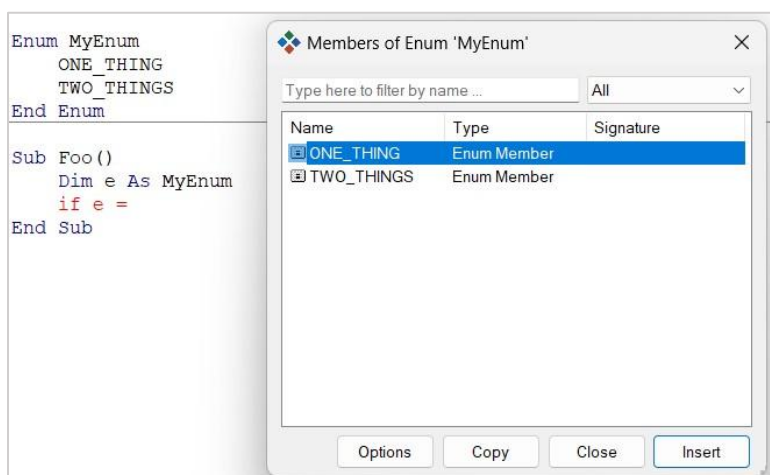
Figure 3 - Enum members
