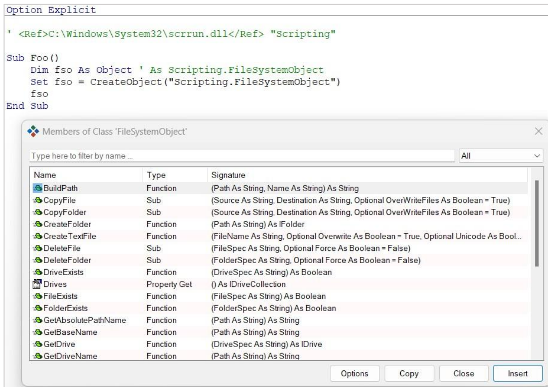
Figure 5 - Special binding
